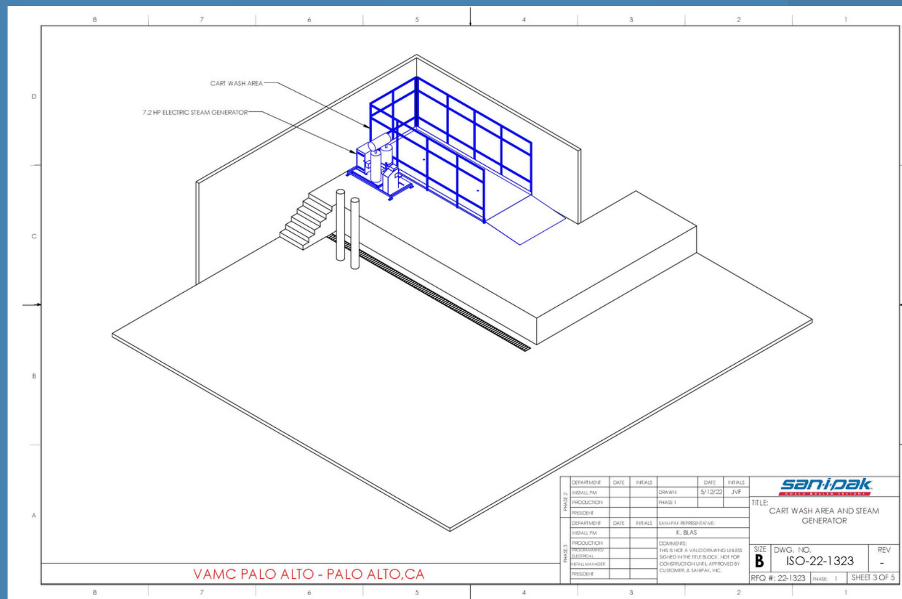
Drawing 2 - ISO
