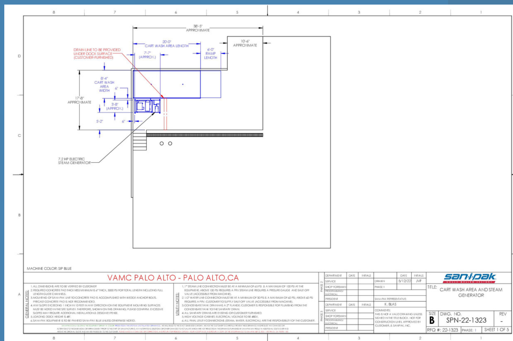
Drawing 1 - Site Plan
